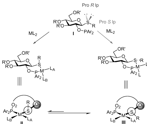
FIGURE 1 Ligand design.
